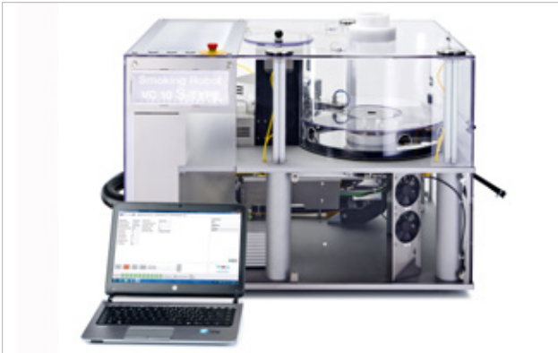
VITROCELL® Smoking Robot VC 10 S-Type Standard version
